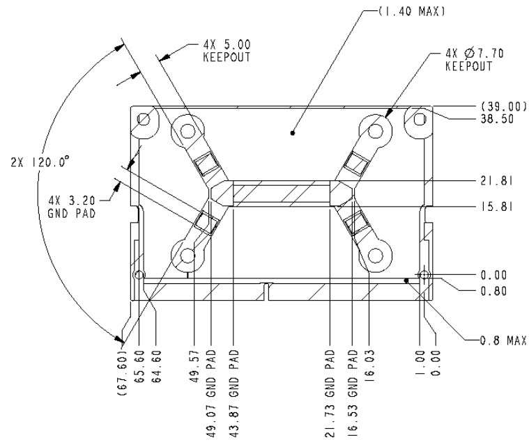
Figure 5-2: Bottom View
